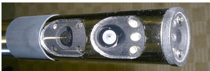
Super Custom Camera head 3 cameras at various FOVs - And angles ie. 0, 45 & 90 degree - in one module Including Lighting
