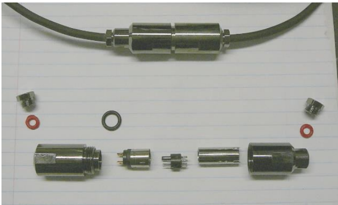
Waterproof - Sealed - Ruggedized Connectors
