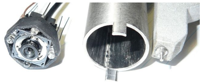
Tiny Custom Focus lens / Camera module for Pipe Tool Fixture
